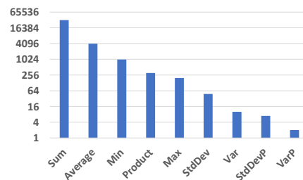
Figure 4: Default Aggregation Functions. (Taking the logarithm of y-axis with base 4)
